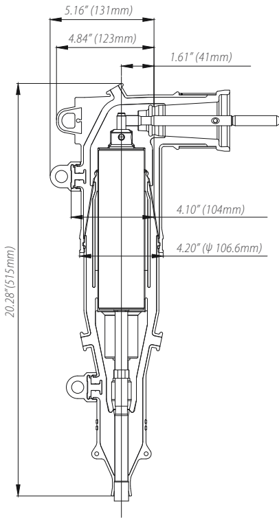
Fig 3: Dimension Info When Hi-Tech Fuse Installed.
