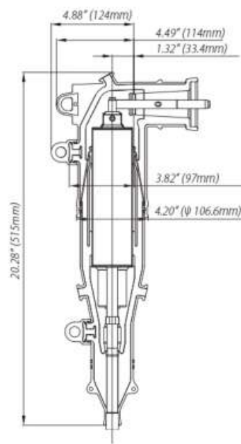
Fig 3: Dimension Info When Hi-Tech Fuse Installed.
